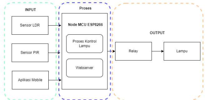
Gambar 2. Blok Diagram
